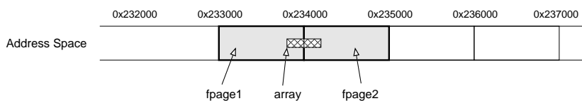
Figure 4.5: An example of making a shared array available using multiple fpages
