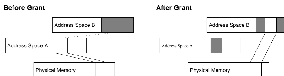
Figure 2.5: A region of one address space is granted to another
